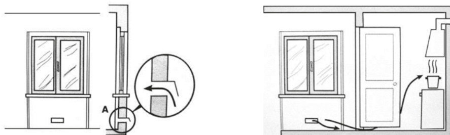
Examples of ventilation holes for combustion air.
